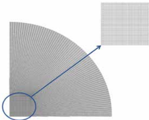
Fig. 3. Finite element mesh for hydraulic bulge test focusing on the central region of the specimen.
