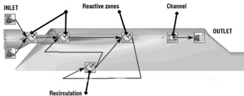
Fig. 1. Equivalent Reactor Networks.
