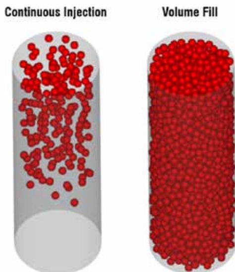
Fig. 2. Particle input method.
