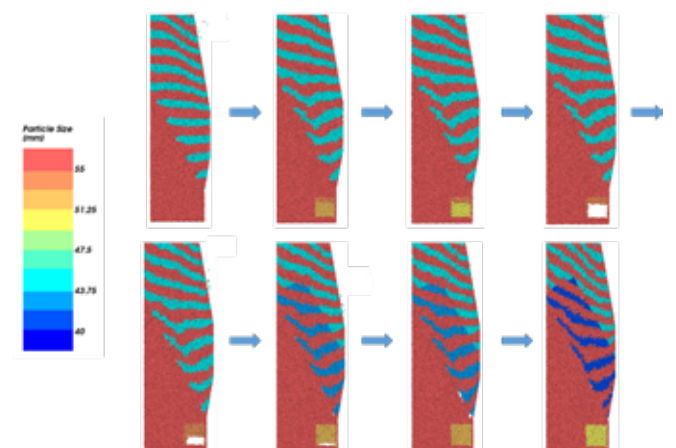
Fig. 7. Particle behaviour inside the blast furnace.
