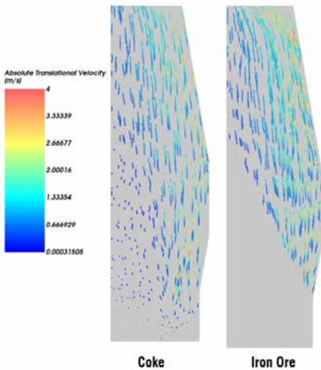
Fig. 8. Particle movement trajectory.
