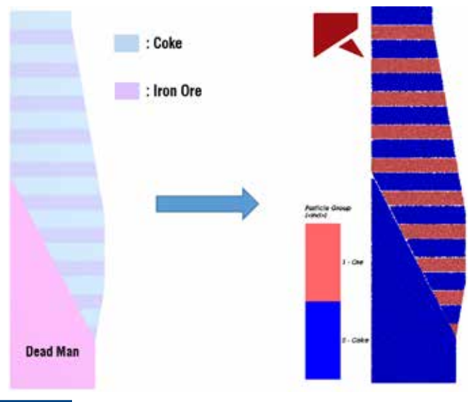
Fig. 3. Initial particle layer placement.
