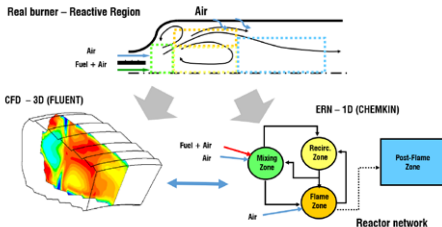
Fig. 2. Burner simulation to link detailed combustion chemistry and CFD.
