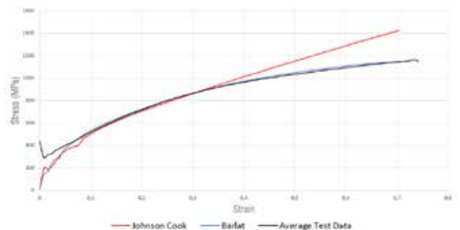
Fig. 6. Comparison of stress-strain results of numerical and experimental hydraulic bulge tests.
