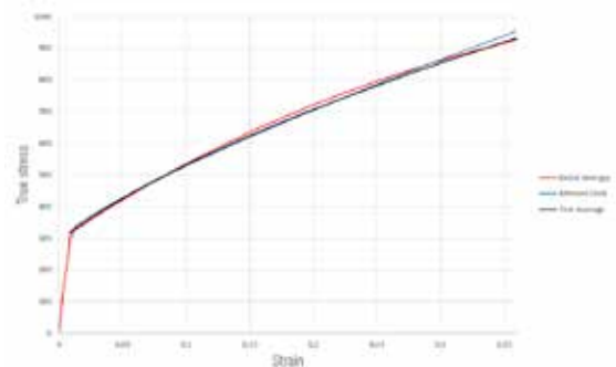
Fig.5. Comparison of stress-strain results of numerical and experimental tensile tests.
