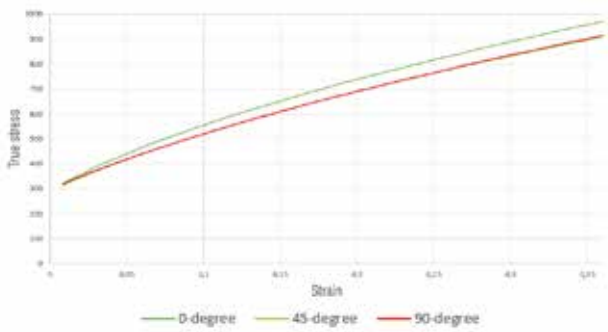
Fig. 1. Tensile test results for roll directions of 0/45/90 degrees.
