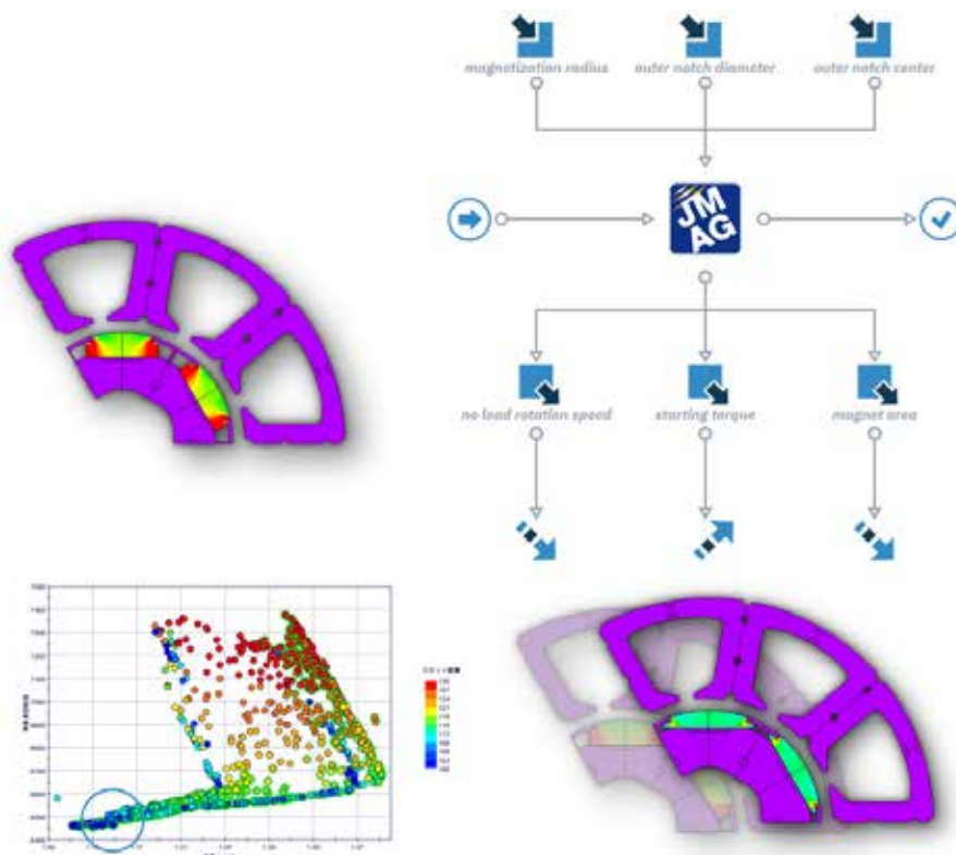
The methodology of combining JMAG-Designer with modeFRONTIER to optimize the permanent magnet rotor for electric motors.
