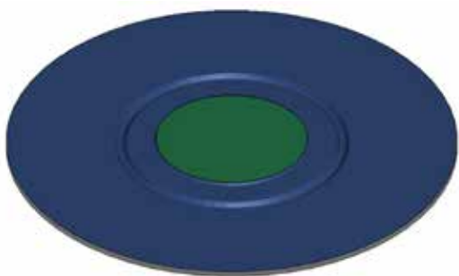
Fig. 4. Numerical model of the hydraulic bulge test.
