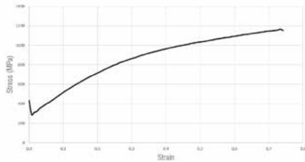
Fig. 2. Result of hydraulic bulge test.
