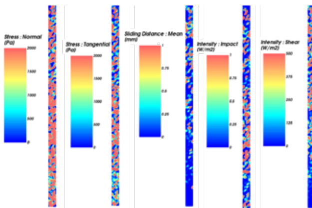
Fig. 9. Example of the structural effect on the blast furnace.
