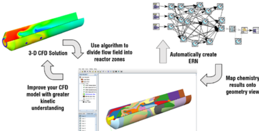
Fig. 4. Automatic generation of an ERN from 3D CFD results using Energico.
