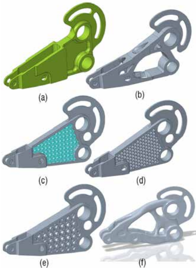
Fig. 5. Multiple feasible generative design solutions for a bell crank. (a) Basic design; (b) results of a traditional topology optimization; (c) beam lattice option; (d) honeycomb filling; (e) gyroid lattice design; (f) high-performance organic generative design solution.
