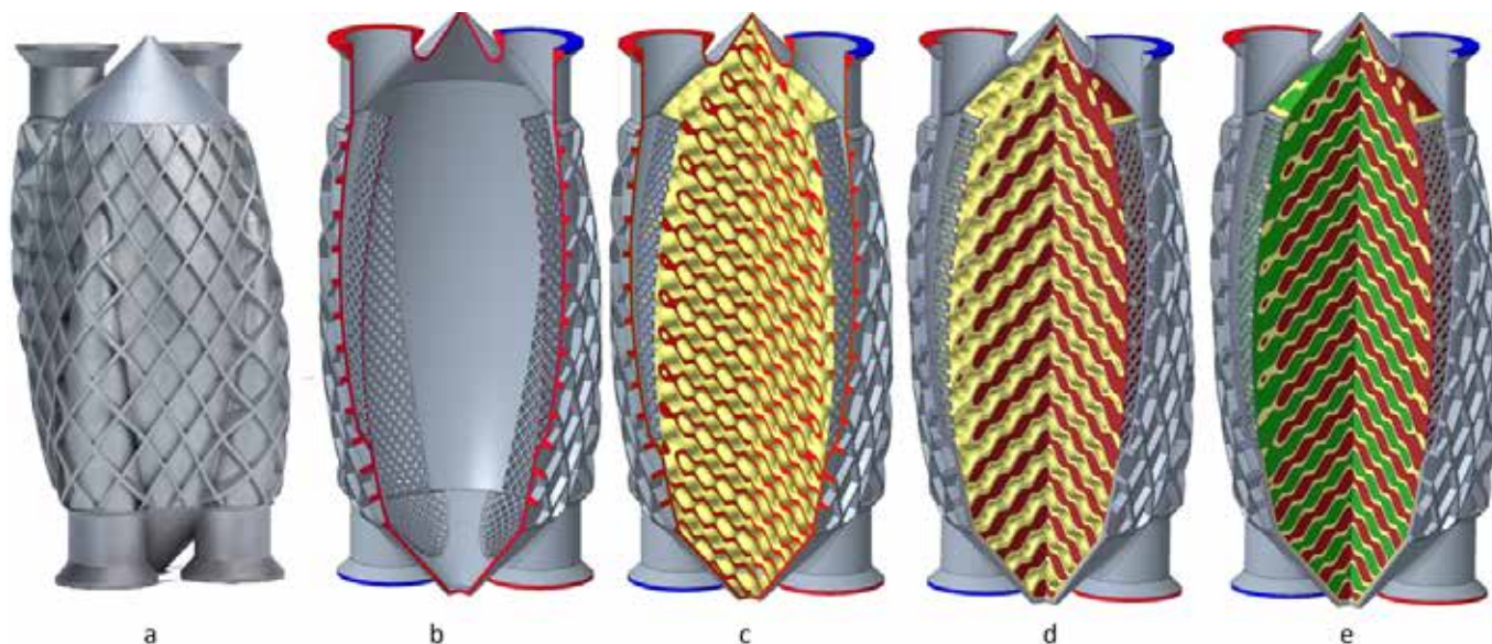
Fig. 4. High-performance avionic heat exchanger. (a) The printed heat exchanger on an EOS M290 printer; (b) the model of the exterior shell structure; (c) with the interior gyroid lattice; (d) with the cold fluid domain; (e) with the hot fluid domain.
