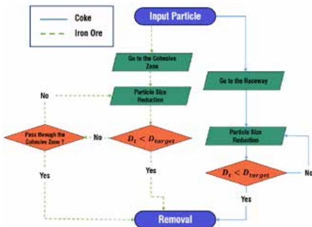
Fig. 5. Flowchart of particle behaviour.
