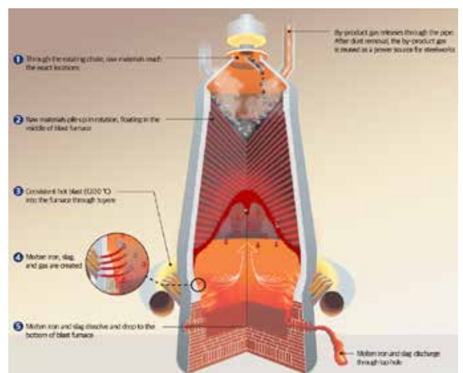
Fig. 1. Blast Furnace. [Courtesy of POSCO Newsroom]
